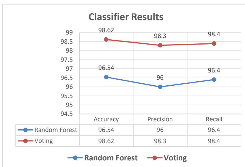
Figure-1: Classifiers Performance
